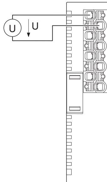
Figure 3 Connecting the sensors
